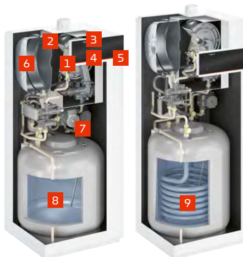
Vitodens 222-F (Type B2TH)
